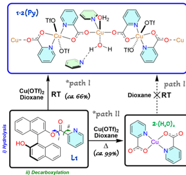
Scheme 5 Proposed pathways L1 \rightarrow 1 \cdot 2(Py) , L1 \rightarrow 2 \cdot (H_2O)_2 , and their relationship with the finding of 1 \cdot (Py) . *Dioxane can absorb water from the reaction medium due to its high solubility and miscibility in water: S(H_2O)^{20^\circ C} = 10^3 \text{ g L}^{-1} .
