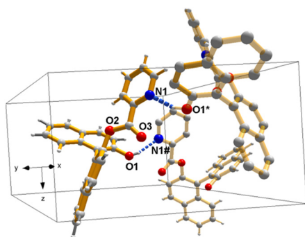
Fig. 1 View of the packing diagram of the benchmark L1 ligand showing the weak interaction ( D-H \cdots A/A: D \cdots A, H \cdots A ): O1-H1 \cdots N1\# :2.799(6), 1.985(5); \{(\#) 1 - y, x - y, 1/3 + z; (*) 1 - x + y, 1 - x, -1/3 + z\} .
