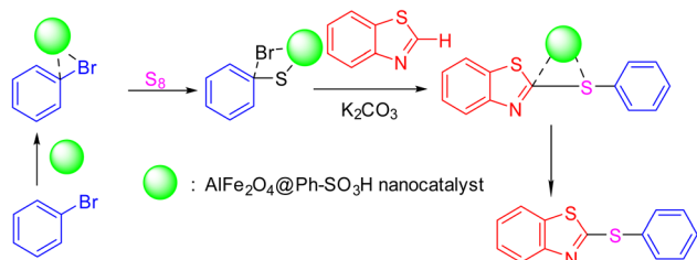
Scheme 3 Suggested mechanism for the synthesis of 2-(phenylthio) benzo[d]thiazole catalyzed by the \text{AlFe}_2\text{O}_4@ \text{SiO}_2\text{-SO}_3\text{H} nanocomposite (product 4a as the model reaction).
