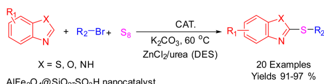
Scheme 2 Synthesis of 2-thioaryl-benzothiazoles, 2-thioaryl-benzoxazoles, and 2-thioarylbenzimidazoles.
