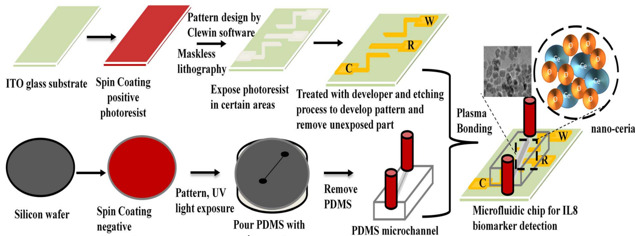
Scheme 1 Steps for the preparation of a microfluidic chip using the maskless lithography technique.
