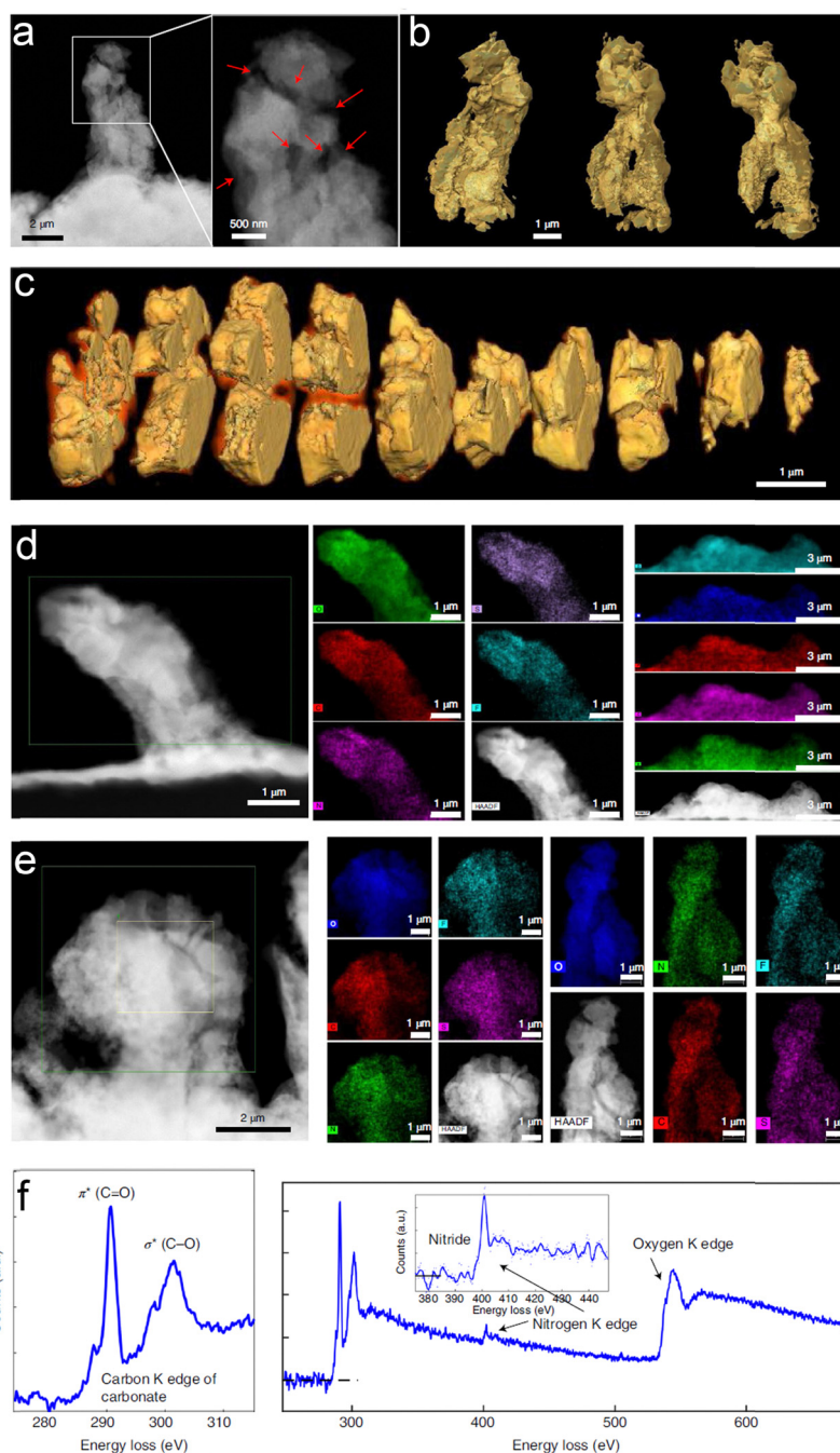
Fig. 19 3D morphology and chemistry of the Li-containing dendrites plated using the baseline succinonitrile-incorporated solid polymer electrolyte (SN-SPE). (a) Cryogenic annular dark-field scanning transmission electron microscopy (ADF-STEM) image and (b) 3D reconstruction of a representative filament obtained by cryogenic tomography based on ADF-STEM images. (c) 3D Cross-section analyses of the filament in (a). (d) and (e) Energy-dispersive X-ray spectroscopy (EDS) maps of several filaments from different regions. The results show that O, C, N, S, and F are distributed throughout the whole filament in all regions. (f) Electron energy-loss spectroscopy (EELS) of the filament. C, N, and O species are identified in the spectra. Reproduced with permission from ref. 147. Copyright 2022, Spring Nature.
