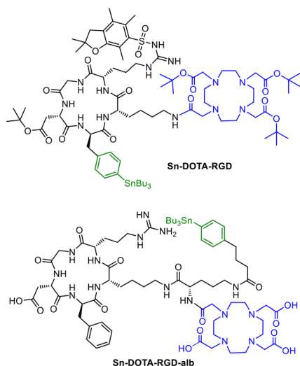
Fig. 8 Molecule structures of the ^t\text{Bu} -protected RGD-stannyl precursor Sn-DOTA-RGD and the stannyl-precursor Sn-DOTA-RGD-alb with albumin binder.
