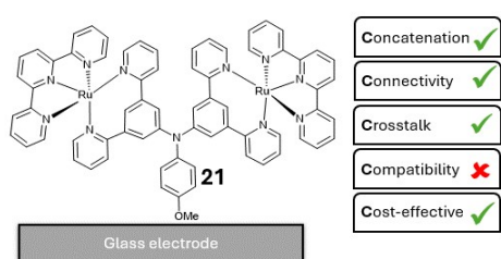
Fig. 20 Molecular logic gate 21 . 59
