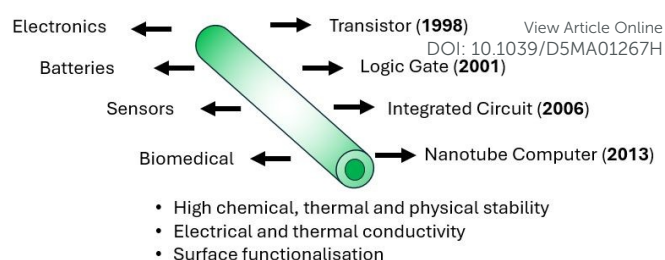
Fig. 31 Nanotube summary.
