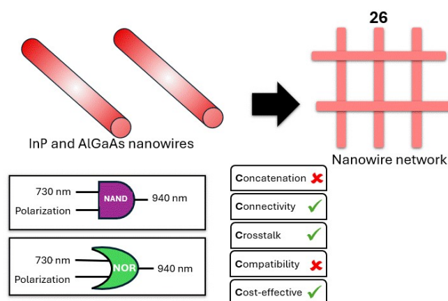
Fig. 28 Nanowire network 26 . 73
