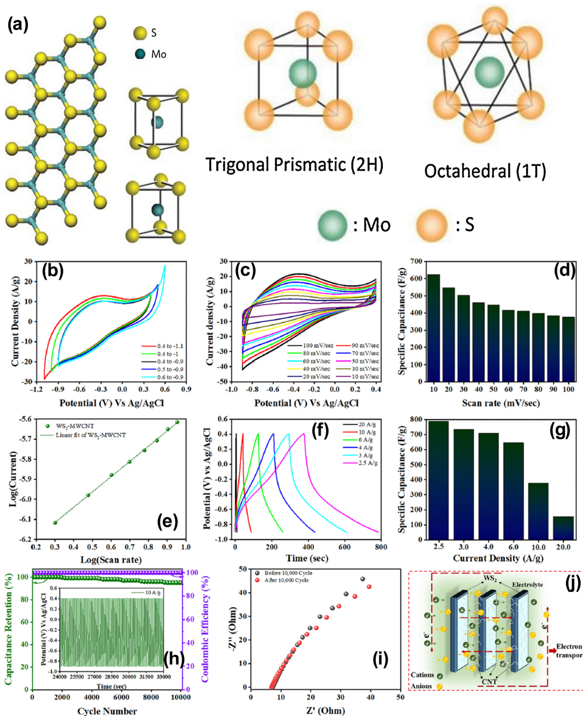
Fig. 6 (a) TMDs crystal structures of \text{MX}_2 and three-dimensional model of the \text{MoS}_2 crystal structure in 1T and 2H types. Reproduced with permission. 194 CV curves of \text{WS}_2 -MWCNT supercapacitor at (b) different potential windows, (c) different scan rates, (d) specific capacitance vs. scan rates bar chart (e) dependency of power law on peak current (f) GCD curves (g) specific capacitance vs. current density bar chart (h) cyclic stability of supercapacitor (i) Nyquist plot before and after 10 000 cycles (j) schematic presentation of \text{WS}_2 -MWCNT supercapacitor. Reproduced with permission. 182
