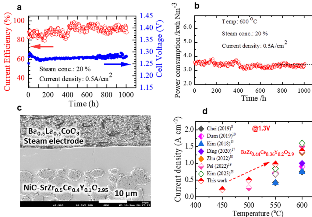
Fig. 6 (a) Long-term durability test of the BSZCY9144362-based cell at 600 °C. (b) Calculated amount of electricity to produce 1 N m³ of H 2 as a function of time. (c) Microstructure of cell post measurement. (d) Performance comparison of our BSZCY44362-based cell with similar electrolyte composition reported in the literature.
