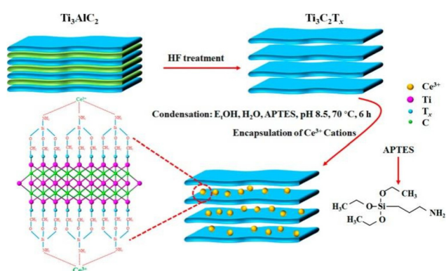
Fig. 10 Schematic illustration of the preparation, surface modification, encapsulation principle and inhibition mechanism of \text{Ti}_3\text{C}_2 MXene- \text{Ce}^{3+} coating. Reproduced with permission 50 from ACS.
