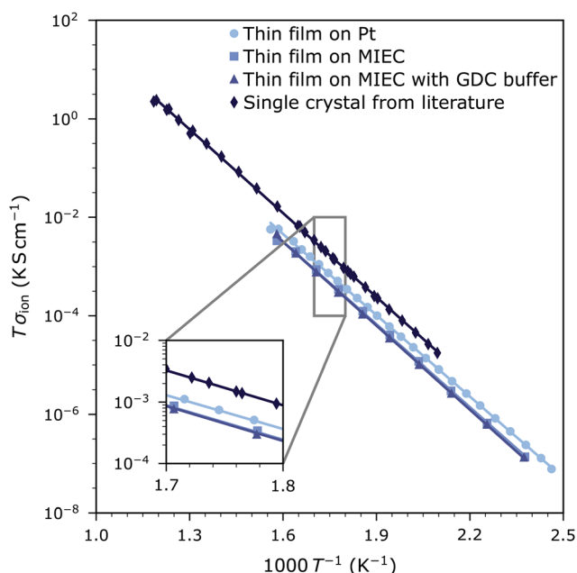
Fig. 6 Ionic conductivity of YSZ thin films prepared by reactive DC sputtering on Pt electrodes and on MIEC perovskite electrodes with and without interfacial GDC buffer layer. The ionic conductivity of a YSZ single crystal is shown for reference. 25
