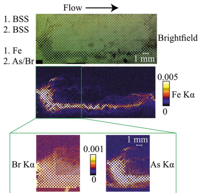
Fig. 11 Scanning \mu XRF within a microfluidic device containing micro-post arrays. Brightfield optical image illustrating the flow direction and chemical addition (top). Model geochemical reactions in the Fe-As-S system are monitored using the appropriate K\alpha fluorescence peak (bottom and insets). Br is utilized as a flow tracer (reproduced with permission from Chen and Kocar, 2021; International Union of Crystallography). 228
