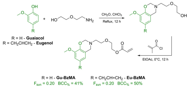
Scheme 4 Synthesis of guaiacol and eugenol-derived acrylate benzoxazines. The bioderived portion of each structure is depicted in green. Re-drawn from ref. 99.
