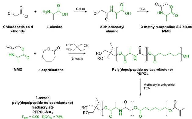
Scheme 11 Synthesis of photocurable PDPCL-MA3. The biobased portion of each structure is depicted in green. TEA = triethylamine, Sn(oct) 2 = tin(II) bis(2-ethylhexanoate). Re-drawn from ref. 172.
