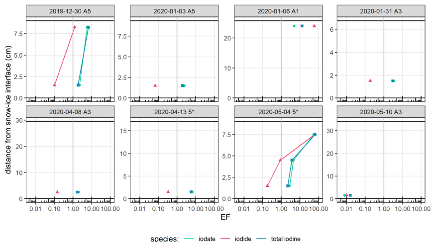
Fig. 4 Enrichment factors (EF) for total iodine, iodide and iodate throughout the snow-pack, for snow over FYI, with respect to sea water. Each panel represents samples taken from an individual snow pit. The height of the snow pit is indicated by the upper black horizontal lines, with the lower line at the snow–ice interface ( h = 0 cm) and the upper line at the snow–air interface (height variable). EFs are displayed on a log scale for total iodine (blue squares), iodide (green circles) and iodide (pink triangles), with a vertical line at EF = 1 as a visual aid. Note the depth scales are variable across snow pits.
