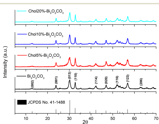
Fig. 1 PXRD patterns of the Bi 2 O 2 CO 3 -based samples.
