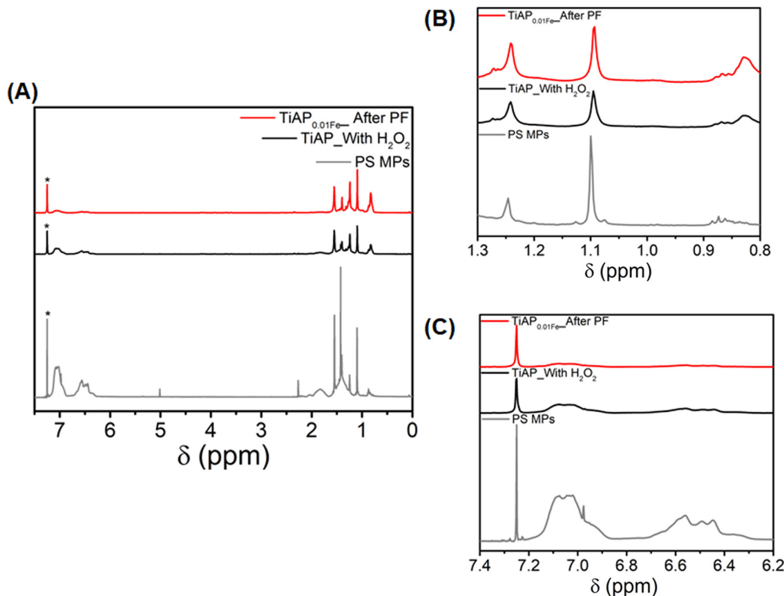
Fig. 5 (A) 1 H NMR spectra of PS MPs, TiAP_With H 2 O 2 , and TiAP 0.01Fe _After PF. (B) and (C) The zoomed-in spectra between 0.8–1.3 ppm and 6.2–7.5 ppm, respectively. Solvent peaks are marked with an asterisk (*).
