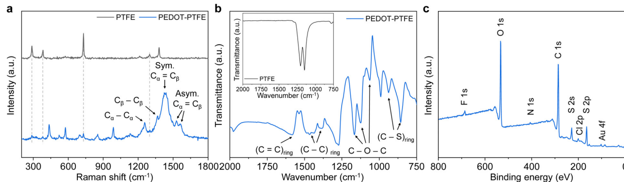
Fig. 2 Spectroscopic characterization of PEDOT-PTFE. (a) Raman spectra of PTFE (black) and PEDOT-PTFE (blue). (b) FTIR spectrum of PEDOT-PTFE. The inset represents the spectrum of pristine PTFE. (c) Survey scan XPS spectrum of PEDOT-PTFE.
