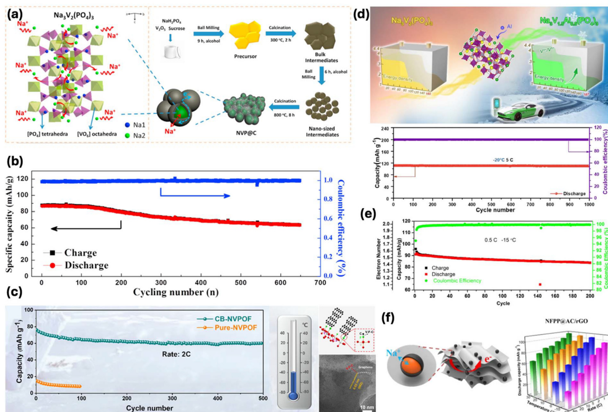
Fig. 10 (a) Schematic representation of Na + transport via hopping mechanism within the crystalline lattice, and synthesis route of the NVP@C nanocomposite. (b) Extended cycling stability of NVP@C evaluated at -20 °C. 38 (c) Cycling performance of the pure NVPOF and CB-NVPOF at -40 °C. 143 (d) Long-term cycling stability of Na 3 V 1.5 Al 0.5 (PO 4 ) 3 at a rate of 5. 145 (e) Cycling performance of NVCP at 0.5C and -15 °C in a three-electrode setup. 146 (f) Bar graph showing NFPP@AC/rGO discharge capacities across various rates and temperatures. 148
