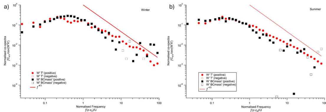
Fig. 1 Co-spectral analysis in winter (194 cases, (a)) and summer (201 cases, (b)) which are binned into 40 evenly spaced bins. BC flux <math>0 \text{ ng}^{-2} \text{ s}^{-1}</math> and u^* < 0.2 \text{ m s}^{-1}</math> co-spectra are removed. Empty marks indicate negative contribution to total flux and are negated when plotting.
