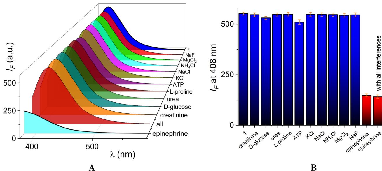
Fig. 7 Fluorescence spectra ( \lambda_{\text{ex}} = 290 \text{ nm} ) (A) and emission intensities at 408 nm (B) of aqueous solutions of 1 ( 5 \mu\text{M} ) containing 10 vol% of \text{CH}_3\text{OH} at pH 7.4 in the presence of various blood plasma and urine components ([interferent] = 1.0 mM, each).
