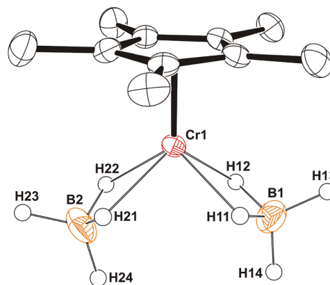
Fig. 4 Perspective view of 7 with thermal ellipsoids at the 50% probability level. Hydrogen atoms of the \eta^5\text{-C}_5\text{Me}_5 ligands are omitted for clarity. Selected lengths (Å): Cr(1)⋯B(1) 2.312(2) , Cr(1)⋯B(2) 2.322(2) , Cr(1)–H 1.82(3) – 1.91(3) , Cr(1)–Cm 1.838 .
