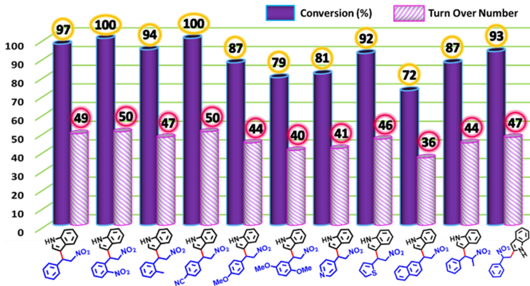
Fig. 4 Substrate scope with substituted \beta -nitrostyrenes showing conversion (%) and turnover numbers obtained under the chosen optimized reaction conditions using the Zn-( p -GluBenz) catalyst.
