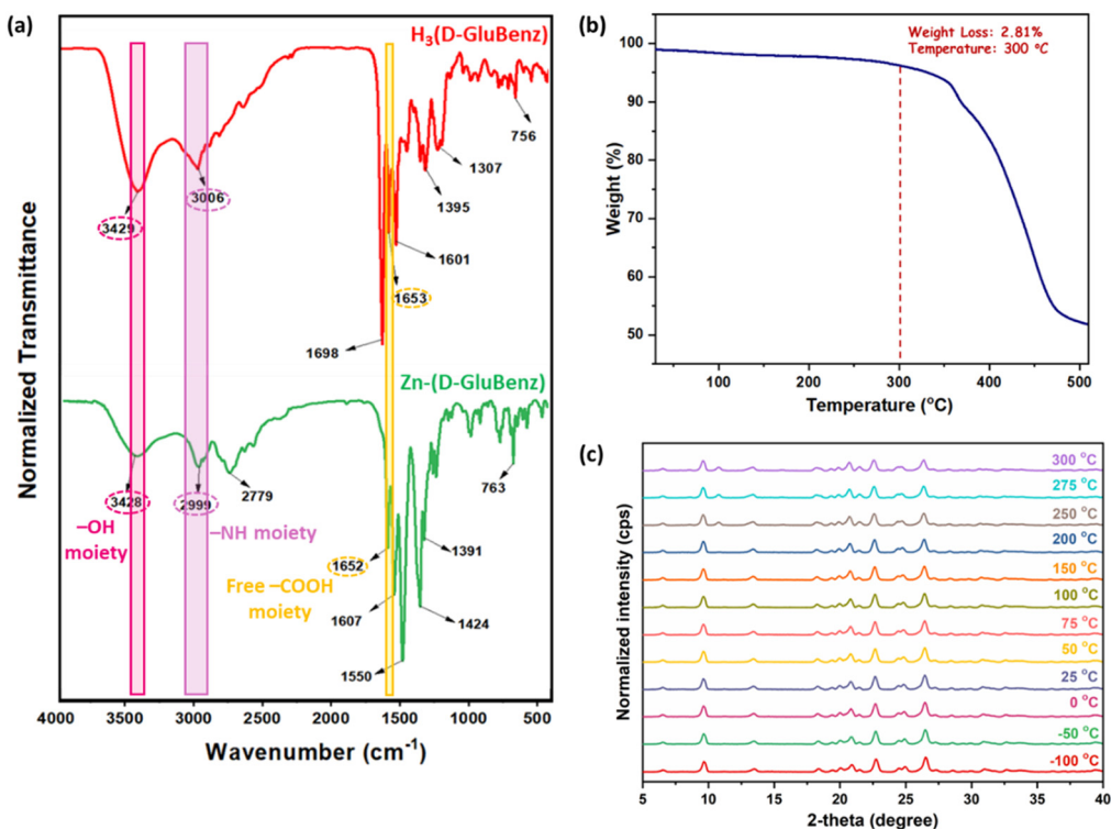
Fig. 1 (a) Comparison of FTIR spectra of \text{H}_3(\text{D-GluBenz}) and Zn-(D-GluBenz) , highlighting the catalytic sites, (b) thermogravimetric analysis profile and (c) VT PXRD patterns from -100 to +300^\circ\text{C} of Zn-(D-GluBenz) .
