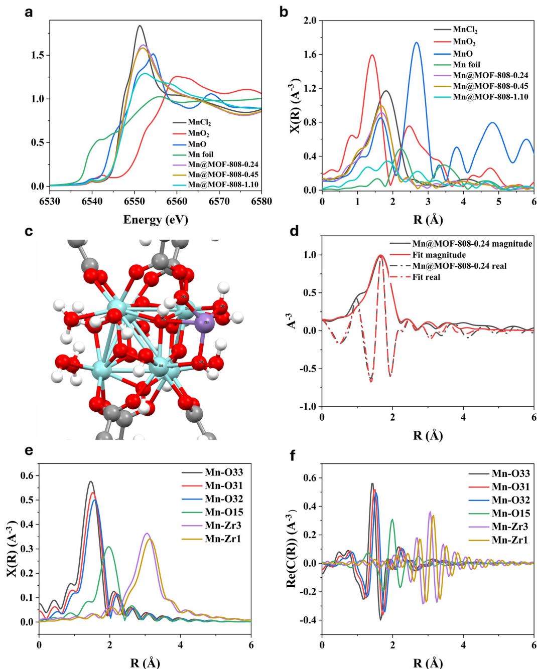
Fig. 2 Mn K-edge (a) XANES and (b) EXAFS spectra of Mn-doped MOF-808 frameworks and \text{MnCl}_2 , \text{MnO}_2 , \text{MnO} and Mn foil references. R -Space EXAFS spectra were obtained from the FT of the k^2 -weighted k -space spectra over a k -range of 3 to 10 \text{ \AA}^{-1} . (c) Model of the Mn@MOF-808 metal cluster (atom colors: teal-Zr, purple-Mn, red-oxygen, gray-carbon, and white-hydrogen). (d) EXAFS fit of Mn@MOF-808-0.24, and the (e) scattering paths contributing to the fit. (f) Real R -space components of selected Mn@MOF-808-0.24 scattering paths.
