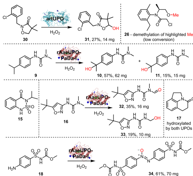
Scheme 3 UPO transformations of amides, ureas and carbamates.
