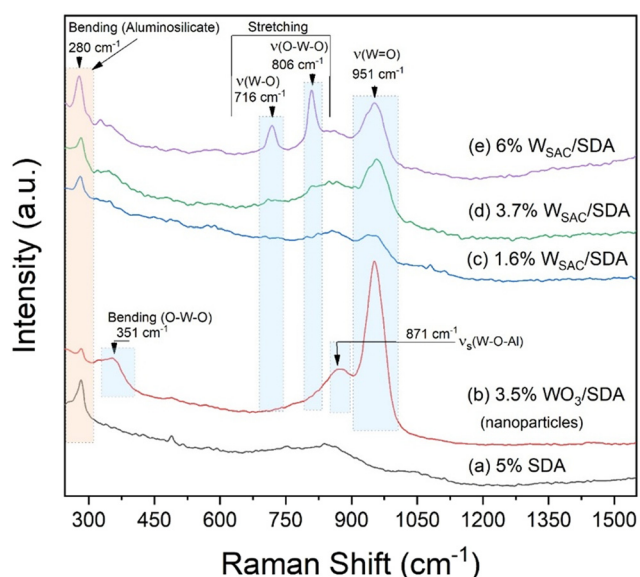
Fig. 2 Raman spectra of (a) the SDA support prepared from SIRAL-5 at 700 °C in air for 5 h, (b) 3.5% WO 3 /SDA nanoparticle catalyst prepared by a sol-gel method without using the templating Zn-MOF, and (c) 1.6 wt%, (d) 3.7 wt%, and (e) 6 wt% W SAC /SDA catalysts prepared using templating Zn-BTC to confine the W 6+ ions and incorporate the isolated W 1 -O 3 moieties within the SDA support.
