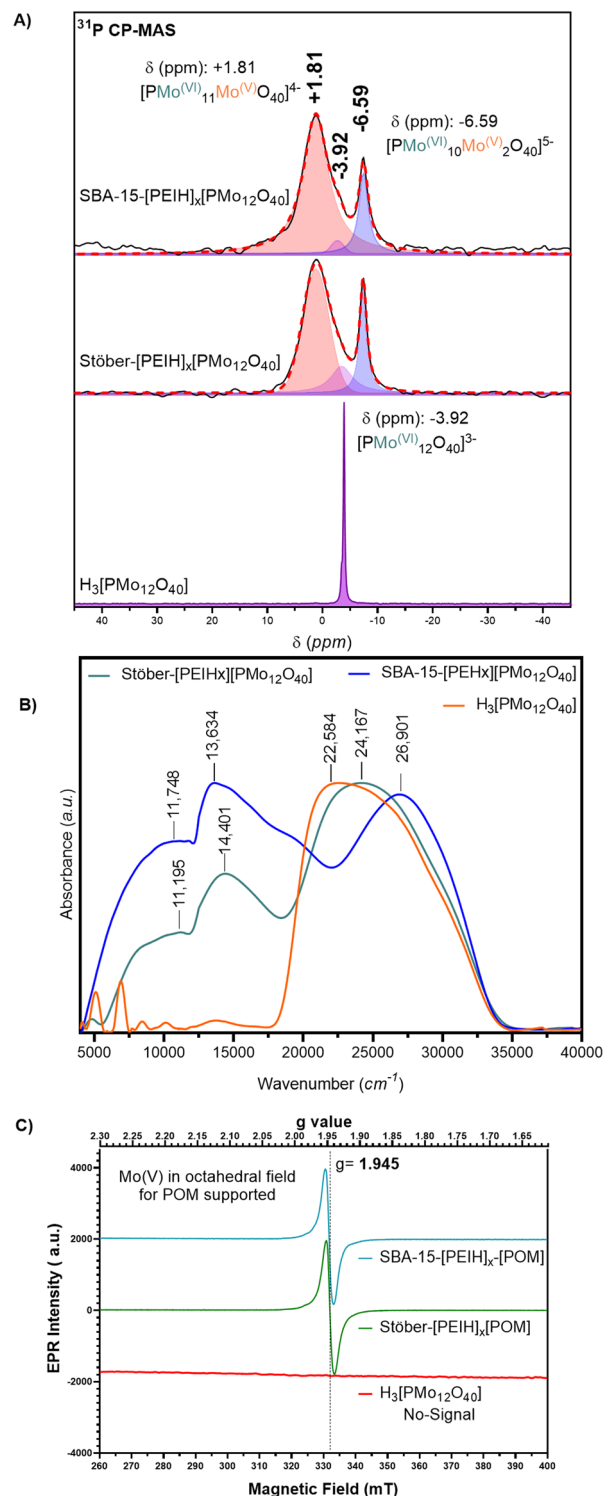
Fig. 4 Spectroscopic characterization of \text{SiO}_2 -[PEI] x [PMo 12 O 40 ]. A) ^{31}\text{P} CP-MAS NMR spectra, B) diffuse reflectance ultraviolet-visible-near infrared spectra, and C) solid state EPR spectra of Mo(v) cations embedded in supported POM clusters at 77 K.
