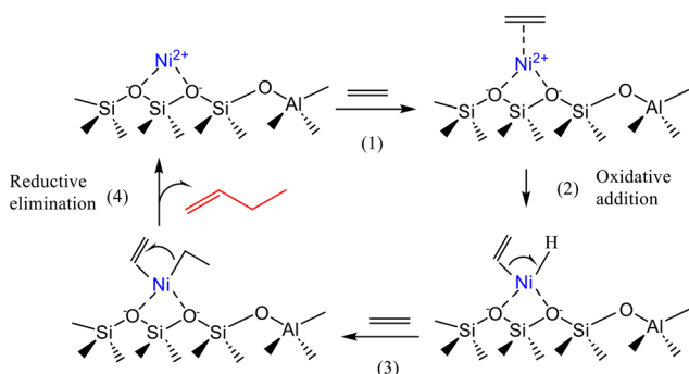
Scheme 6 Simplified catalytic cycle proposed for the activation and dimerization of ethylene on the active Ni 2+ centers of Ni-Beta catalysts: (1) ethylene adsorption on Ni site; (2) oxidative addition; (3) ethylene insertion; (4) reductive elimination of butene. This scheme has been adapted from ref. 7 with permission from American Chemical Society, copyright 2025.
