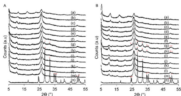
Fig. 4 PXRD patterns of wHf-LFS50s (A) and wHf-LFS150s (B). (A) 8Hf-LFS50-Na (WI (a); SS (b)); 8Hf-LFS50-TPA (WI (c); SS (d)); 8Hf-LFS50-HT (WI (e); SS (f)); wHf-LFS50-SS ( w = 16 (g), 12 (h), 8 (i), 4 (j), 2 (k)); wHf-LFS50-WI ( w = 8 (l), 2 (m)); \text{HfO}_2 (n). (B) 8Hf-LFS150-Na (WI (a); SS (b)); 8Hf-LFS150-TPA (WI (c); SS (d)); 8Hf-LFS150-HT (WI (e); SS (f)); wHf-LFS150-SS ( w = 16 (g), 12 (h), 8 (i), 4 (j), 2 (k)); wHf-LFS150-WI ( w = 8 (l), 2 (m)); \text{HfO}_2 (n).
