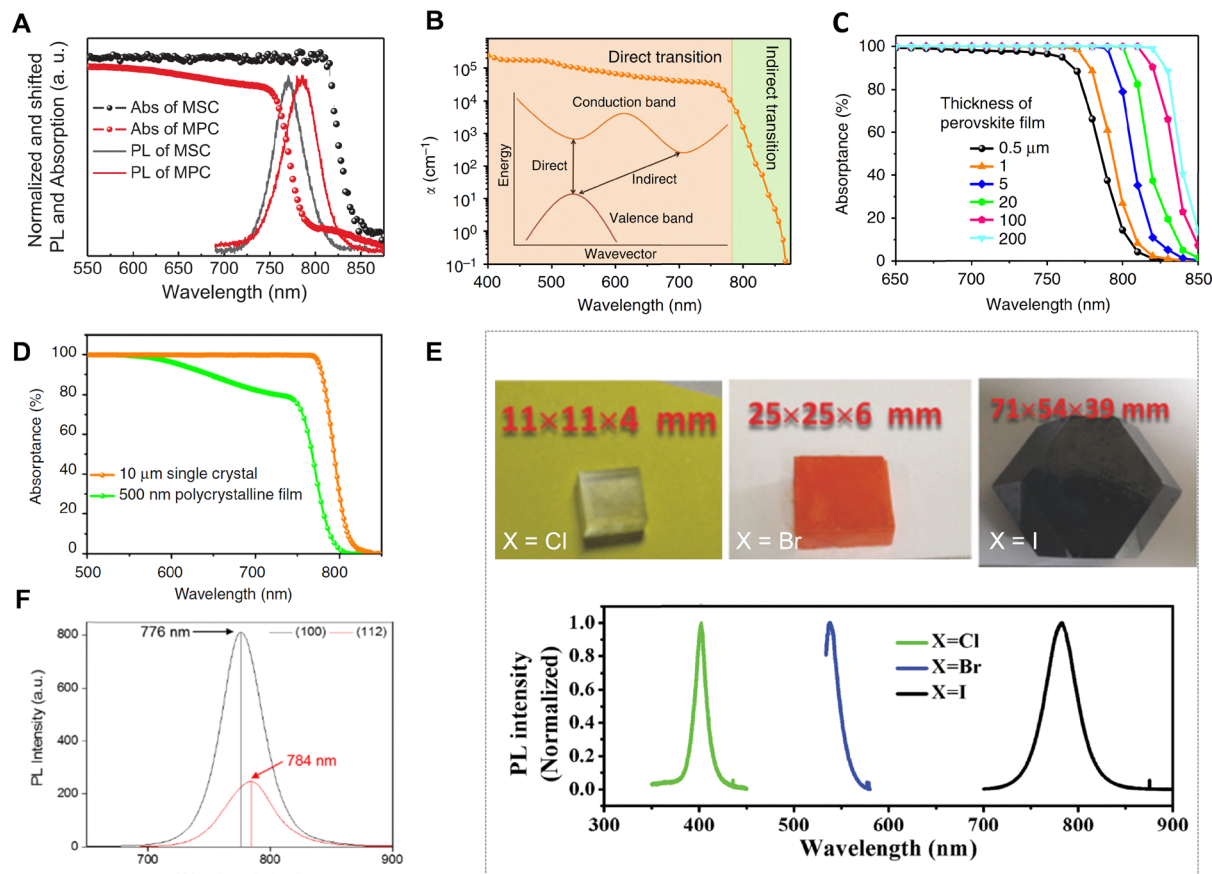
Fig. 2 (A) Normalized PL and absorption spectra of the \text{MAPbI}_3 single crystals (MSCs) and \text{MAPbI}_3 polycrystalline (MPC) thin films. Reproduced with permission from ref. 48, Copyright 2015, The American Association for the Advancement of Science. (B) Schematic illustration of direct and below-bandgap transitions, along with the absorption coefficient of a polycrystalline \text{MAPbI}_3 film. (C) The calculated absorption of \text{MAPbI}_3 films with different thickness. (D) Absorption spectra of a 10- \mu\text{m} -thick \text{MAPbI}_3 thin single crystal and a 500-nm-thick polycrystalline film. Reproduced with permission from ref. 67, Copyright 2017, Springer Nature. (E) Photographs of as-grown \text{CH}_3\text{NH}_3\text{PbX}_3 ( X = \text{Cl, Br, I} ) single crystals and their corresponding PL spectra. Reproduced with permission from ref. 75, Copyright 2015, Wiley-VCH Verlag GmbH & Co. KGaA, Weinheim. (F) PL spectra of (100) and (112) facets of SC \text{MAPbI}_3 . Reproduced with permission from ref. 72, Copyright 2019, American Chemical Society.
