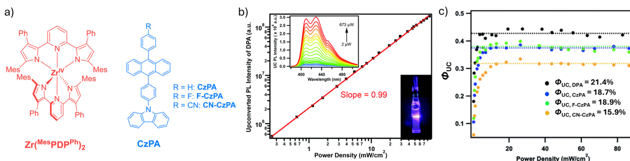
Fig. 11 Green-to-blue upconversion sensitized by Zr(MesPDPPh) 2 with DPA and carbazole-based DPA derivatives (CzPA) as the annihilator. 175 (a) Molecular structures of Zr(MesPDPPh) 2 and the CzPA annihilators. (b) Double logarithmic plot of integrated upconversion luminescence intensity for the Zr(MesPDPPh) 2 /DPA (0.25 mM) pair in deaerated THF as a function of the excitation power density at 514 nm, and the corresponding upconversion luminescence spectra (upper inset). Bottom inset: Image of the upconversion sample under 514 nm irradiation. (c) Upconversion quantum yields (theoretical maximum set to 50% 54 ) determined with a Zr(MesPDPPh) 2 photosensitizer and DPA or CzPAs annihilator in deaerated THF, plotted as a function of the excitation power density at 514 nm. 175 Reproduced under terms of the CC-BY license from ref. 175. Copyright 2021, Royal Society of Chemistry.
