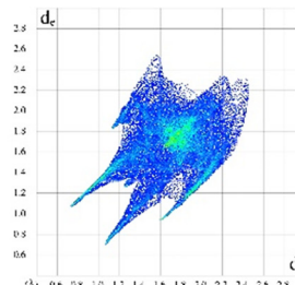
Fig. 5 Hirshfeld surfaces with short intermolecular contacts (red spots) in (a) 1, (b) 2, (c) 3, and (d) 4 (two perpendicular views). In the right column, 2D fingerprint plots of main contacts are represented.
