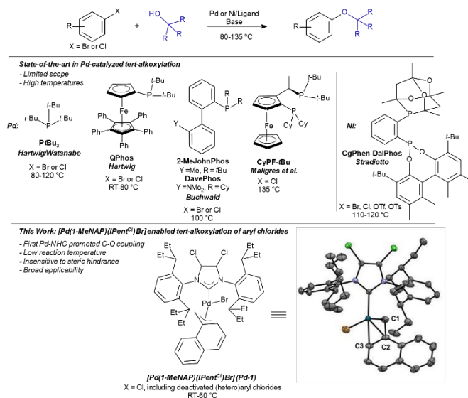
Scheme 1. Catalytic couplings of aryl halides with tertiary alcohols. In the depicted X-ray of the [Pd(1-MeNAP)(IPent Cl )Br] catalyst, displacement ellipsoids are shown at the 50% probability level, hydrogens are omitted for clarity (CCDC = 2492026). Selected bond lengths (Å): C NHC -Pd = 2.049(3), Pd-C1 = 2.092(3), Pd-C2 = 2.242(3), Pd-C3 = 2.267(3).
