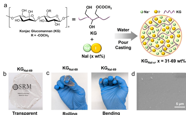
Fig. 1 (a) Synthetic scheme for the preparation of solid-state electrolyte films ( \text{KG}_{\text{NaI}-x} ; x = 31\text{--}69 wt%). (b) An image of a representative transparent film of \text{KG}_{\text{NaI}-69} . (c) Photographs of two different modes of flexibility of a representative \text{KG}_{\text{NaI}-69} film. (d) Scanning electron microscope image of \text{KG}_{\text{NaI}-69} film. Scale bar: 5\ \mu\text{m} .
