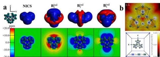
Fig. 8 (a) Isosurface and contour plot representation of the magnetic response properties for [\text{Co}_3\text{@Ge}_6\text{Sn}_{18}]^{5-} , denoting the NICS (isotropic/averaged) term, and from different orientations of the external field ( B_x^{\text{ind}} , B_y^{\text{ind}} , and B_z^{\text{ind}} ). Isosurfaces set to \pm 8 ppm, blue: shielding; red: deshielding. (b) Current density of the [\text{Co}_3\text{@Ge}_6\text{Sn}_{18}]^{5-} cluster at the central plane located at 0 Å, containing the [\text{Co}_3\text{Ge}_3] ring. The calculations were performed at the PBE0/def2-TZVP level of theory, without including solvent effects. Reprinted with permission from ref. 210. Copyright 2025 American Chemical Society.
