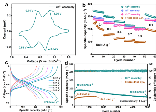
Fig. 2 (a) CV profile. (b) The corresponding rate performance profiles of \text{Co}^{2+} , \text{Ni}^{2+} , and \text{Cu}^{2+} cathodes. (c) The corresponding GCD profiles at various current densities of the \text{Co}_{0.14}\text{V}_2\text{O}_5 \cdot 0.95\text{H}_2\text{O} cathode. (d) Long-term cycling stability at 5.0 \text{ A g}^{-1} of \text{Co}_{0.14}\text{V}_2\text{O}_5 \cdot 0.95\text{H}_2\text{O} and freeze-dried \text{V}_2\text{O}_5 cathodes.
