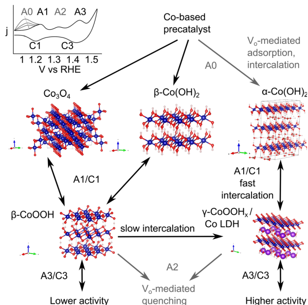
Scheme 2 The surface reconstruction pathways followed by Co-based OER catalysts. Oxygen is shown in red, hydrogen in cream, and cobalt in blue. \alpha\text{-Co(OH)}_2 is intercalated by water and anions (i.e. \text{CO}_3^{2-} with C shown in brown), whereas \gamma\text{-CoOOH}_x is intercalated by cations (i.e. \text{K}^+ shown in purple). 61 \text{Co}_3\text{O}_4 , 64 \beta\text{-Co(OH)}_2 , 65 \beta\text{-CoOOH}_x , 66 data accessed via the Crystallography Open Database. Note that the more active intermediate form of \gamma\text{-CoOOH}_x vs. a Co layered double hydroxide (LDH) structure is not yet fully clear and may be material specific.
