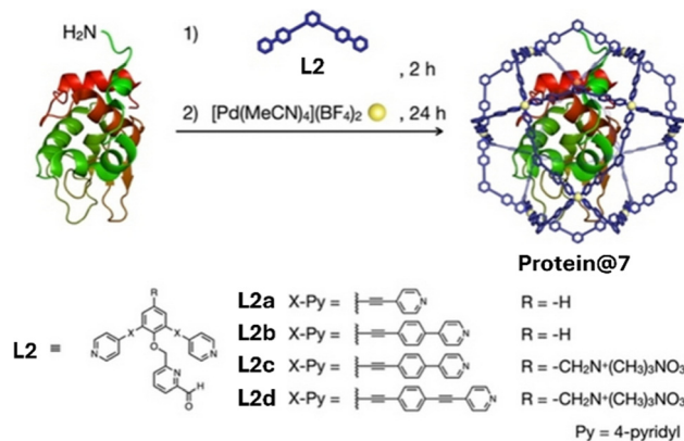
Fig. 5 Encapsulation of a protein within a M 12 L 24 MOC (7) and the range of linkers (L2a–d) employed to generate isostructural cages with a range of internal void cavities. Reproduced with permission from ref. 22.
