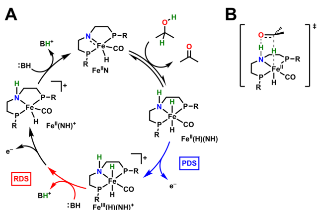
Fig. 4 (A) Catalytic cycle of Fe-pincer complex, FeN , proposed in McLoughlin et al. (R = iPr 2 , B = P 2 -Et). (B) Six-membered transition state involving a 2H + /2e − transfer between acetone to the metal center and PNP ligand.
