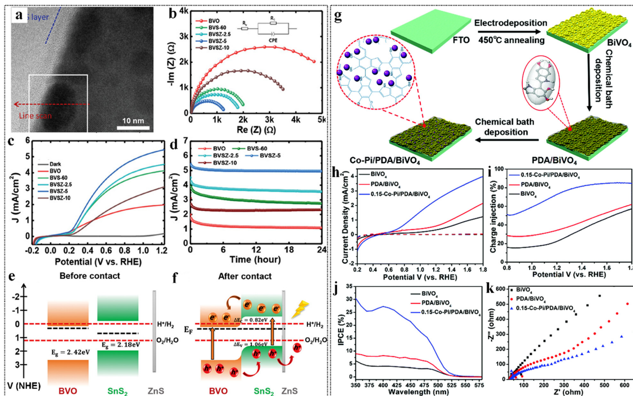
Fig. 4 (a) A BFTEM cross-sectional image for a \text{BiVO}_4 film with embedded \text{SnS}_2 nanoparticles and a \text{ZnS} coating layer. (b) EIS Nyquist plots, (c) LSV curves, and (d) stability curves for the BVO, BVS-60, BVSZ-2.5, BVSZ-5, and BVSZ-10 photoanodes. (e) and (f) Band diagrams of a BVO/ \text{SnS}_2 / \text{ZnS} photoanode before and after contact. Reproduced from ref. 96 with permission from Wiley, copyright 2024. (g) Synthesis of Co-Pi/PDA/ \text{BiVO}_4 . (h) J–V plots of \text{BiVO}_4 , PDA/ \text{BiVO}_4 , and 0.15-Co-Pi/PDA/ \text{BiVO}_4 . (i) Charge injection efficiencies. (j) IPCE spectra. (k) PEIS plots of \text{BiVO}_4 , PDA/ \text{BiVO}_4 , and 0.15-Co-Pi/PDA/ \text{BiVO}_4 . Reproduced from ref. 98 with permission from Royal Society of Chemistry, copyright 2019.
