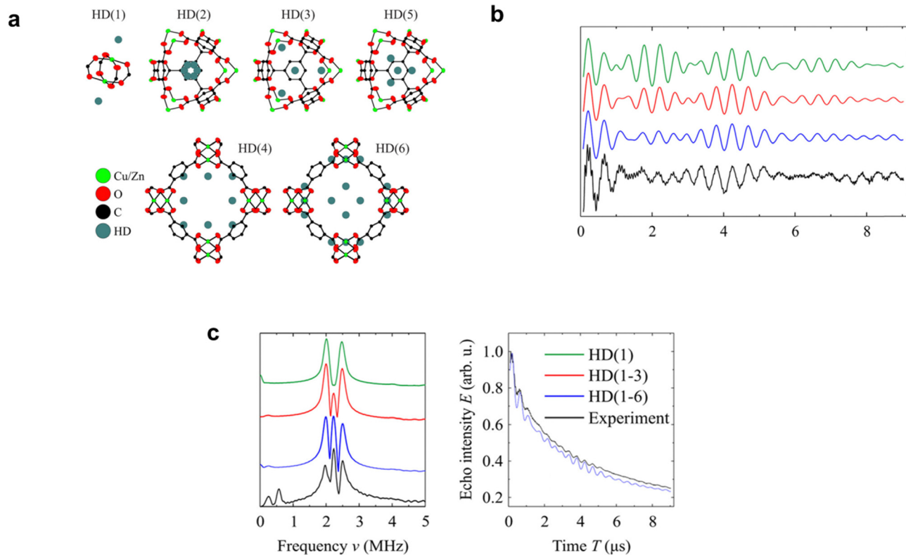
Fig. 8 (a) Variations of HD adsorption sites in \text{Cu}_3(\text{btc})_2 as determined from NPD experiments. 46 Normalized (b) baseline-corrected time domain and (c) corresponding frequency domain 3p ESEEM simulations for different expected HD sites in \text{Cu}_{2.97}\text{Zn}_{0.03}(\text{btc})_2 . The experimental 3p ESEEM data recorded at 6 K are given for comparison. In addition, experimental and simulated TD traces with recovered decaying baseline are also provided. Reproduced with permission from ref. 27 Copyright 2015 American Chemical Society.
