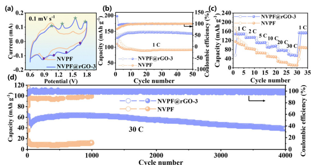
Fig. 3 (a) CV curves at 0.1 \text{mV s}^{-1} . (b) Cycling performance at 1C. (c) Rate performance. (d) Cycling performance at 30C.
