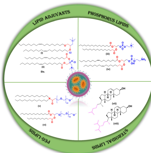
Fig. 3 The types of lipids contained in the LNP formulations, (i) DOTMA, (ii) (R)-DOTAP, (iii) 1,2-distearoyl- sn -glycero-3-phosphocholine (DSPC), (iv) DOPE, (v) (4-hydroxybutyl)azanediybis(hexane-6,1-diyl)bis(2-hexyldecanoate)(ALC-0159), (vi) 1,2-dimyristoyl- rac -glycero-3-methoxypolyethylene glycol-2000(PEG-DMG-2000), (vii) cholesterol, and (viii) β-sitosterol.
