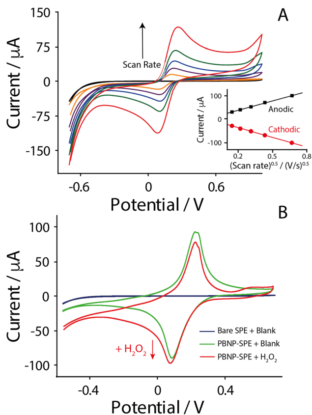
Fig. 2 (A) CV curves of screen-printed electrodes at various scan rates ranging from 0.02 to 0.5 V s -1 in a solution containing 5 mM potassium ferricyanide (K 3 Fe(CN) 6 ) in 0.1 M KCl. (Inset) anodic and cathodic peak currents versus the square root of the scan rate of the electrode confirming diffusion-controlled redox behavior, consistent with the Randles-Ševčík equation. (B) Comparative CV curves obtained in 0.1 mol per L KCl solution of bare SPE (blue), SPE modified with 10 mM PB (green), and SPE modified with PB in the presence of 5 mmol per L H 2 O 2 (red). Experimental parameters: starting potential: -0.7 V; first vertex potential (E V1 ): -0.7 V; second vertex potential (E V2 ): 0.7 V; potential step (E step ): 0.01 V; scan rate: 0.1 V s -1 ; no. of scans: 2.
