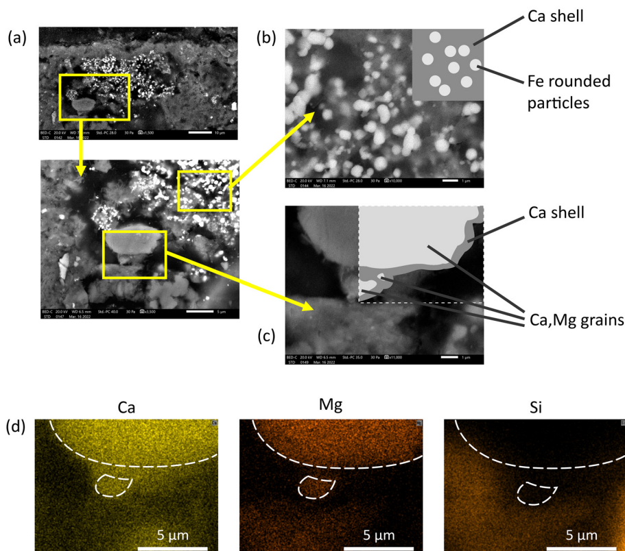
Fig. 7 Sample S2. Crystallization of new phases in correspondence to the Fe-based pigments and Ca- and Mg- agglomerates. (a) SEM BES images of layer 3; (b) detail of the SEM BES images at a higher magnification and the scheme (on the top right) showing the rounded morphology of the Fe-based particles of the pigment (in light grey) and the Ca-based newly formed network composed of micrometric and submicrometric middle grey crystallites having a plate-like or needle-like morphology; (c) detail of the SEM BES images at a higher magnification and the scheme (on the top right) of Ca- and Mg-containing grains surrounded by the newly-formed Ca-based shell; and (d) elemental distribution maps of calcium (Ca), magnesium (Mg) and silicon (Si). The dotted white lines mark the boundaries of the Ca and Mg grains and highlight the surrounding Ca-based shell.
