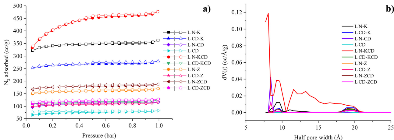
Fig. 4 (a) N_2 adsorption/desorption isotherms of lignin-based activated porous carbons at -196^\circ\text{C} (solid symbols represent adsorption and hollow symbols indicate desorption), and (b) pore size distribution from the NLDFT method using N_2 isotherms at -196^\circ\text{C} .
