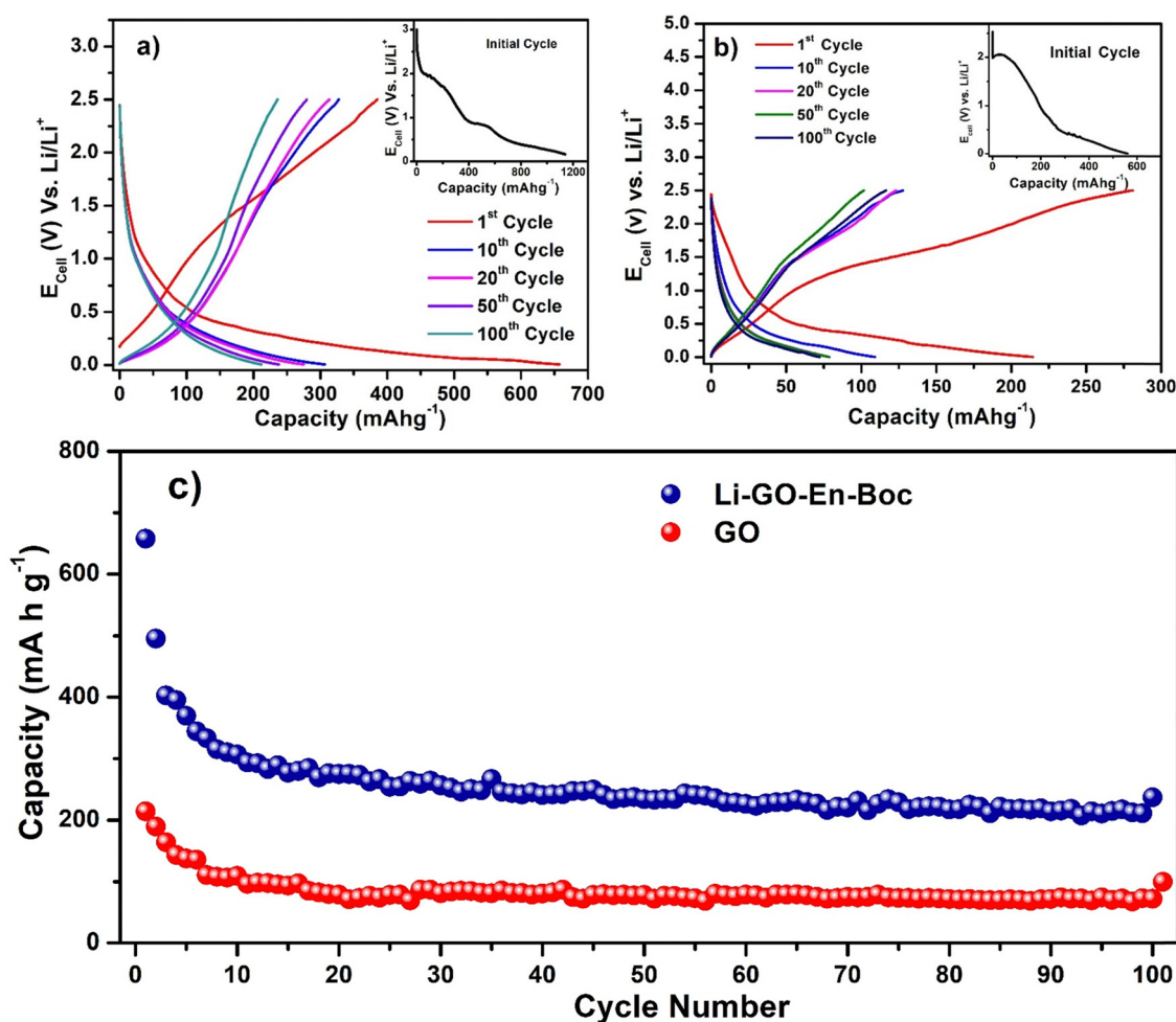
Fig. 7 Charge–discharge profiles for (a) Li-GO-EnBoc and (b) GO electrode cycled at 25 \text{ mA g}^{-1} between 2.5 and 0.005 V vs. \text{Li}/\text{Li}^+ in 1 M \text{LiPF}_6 in a 1:1 (v/v) mixture of ethylene carbonate (EC) and dimethyl carbonate (DMC) as the electrolyte. (c) Variation in discharge capacity vs. cycle number for GO and Li-GO-EnBoc.
