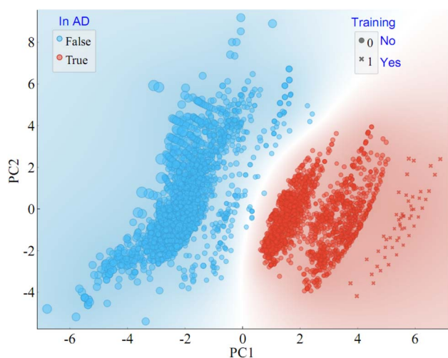
Fig. 6 The application domain of the MLR model is characterised by a PCA-based approach for the LC-RT of PFAS. Chemicals in AD are shown in red, otherwise in blue; chemicals in the training dataset are in 'x' shape, otherwise in dot shape; the size of the symbols represents the Euclidean distance.
