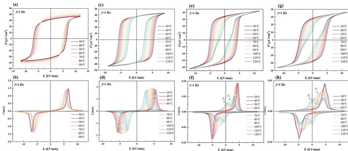
Fig. 6 Temperature-dependent (a) P - E loops and (b) I - E curves of the BNT-88 \mu\text{m} MLCC at 12 \text{ kV}/\text{mm}^{-1} ; (c) P - E loops and (d) I - E curves of the BNT-78 \mu\text{m} MLCC at 9 \text{ kV}/\text{mm}^{-1} ; (e) P - E loops and (f) I - E curves of the BNT-35 \mu\text{m} MLCC at 12 \text{ kV}/\text{mm}^{-1} ; (g) P - E loops and (h) I - E curves of the BNT-28 \mu\text{m} MLCC at 12 \text{ kV}/\text{mm}^{-1} .
