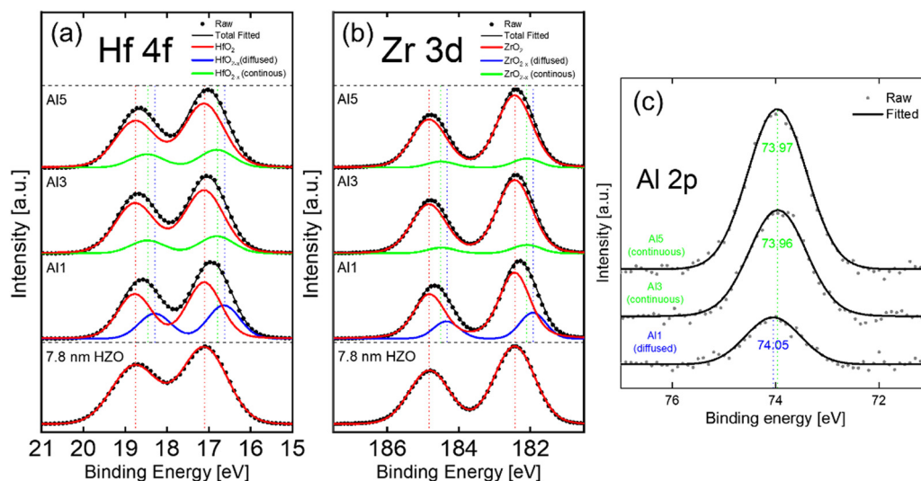
Fig. 5 The baseline subtracted XPS spectra of (a) Hf 4f, (b) Zr 3d, and (c) Al 2p of the Al1, 3, and 5(7.8 nm). The Hf 4f and Zr 3d spectra of the sample without interlayer are also compared.
