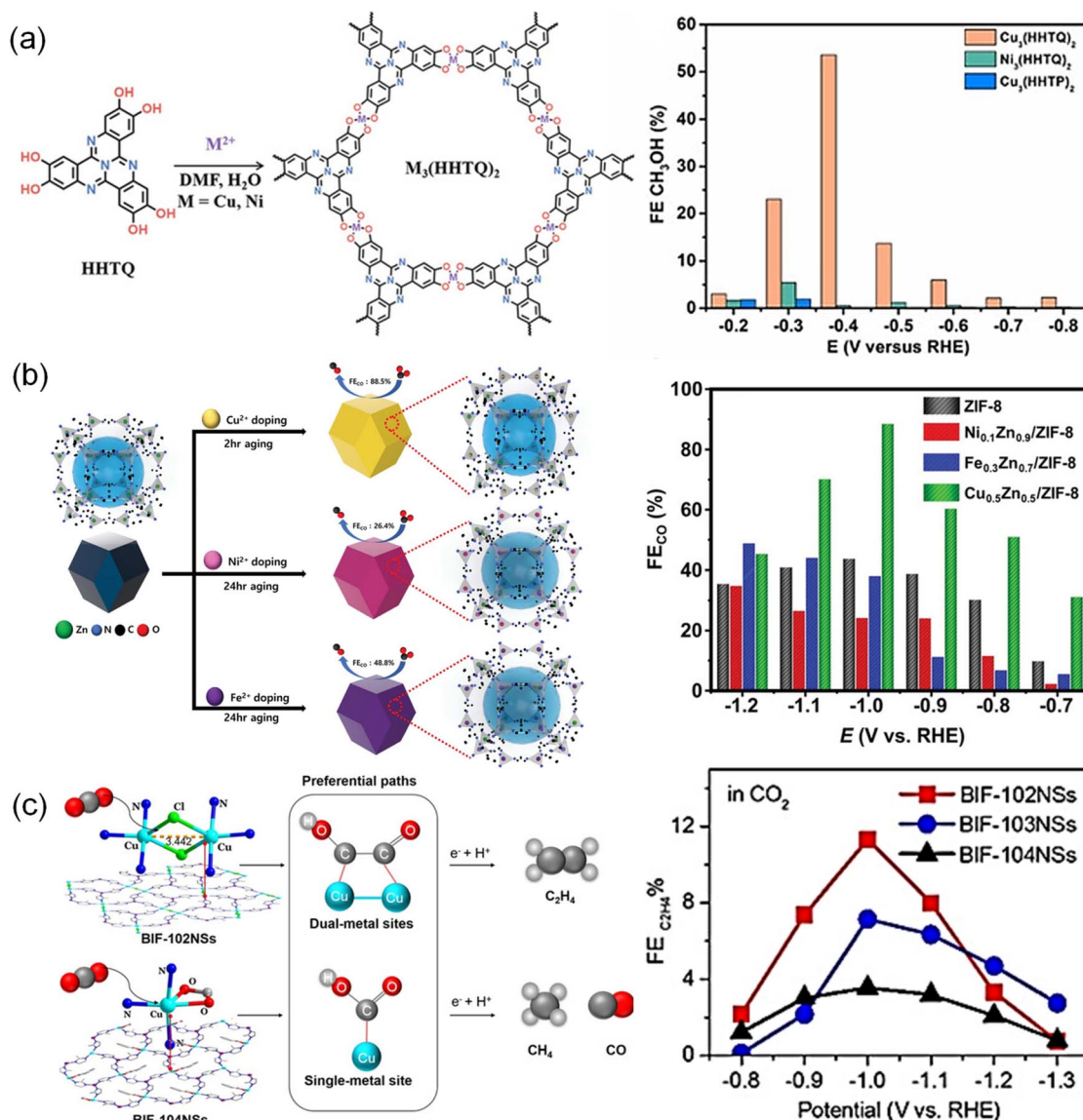
Fig. 3 (a) Schematic synthesis of M_3(\text{HHTQ})_2 ( M = \text{Cu, Ni} ) and FE of \text{CH}_3\text{OH} . 138 Copyright 2021, Wiley-VCH. (b) Schematic synthetic strategy of the M_xZn_y/\text{ZIF-8} catalyst and FE of \text{CO} . 69 Copyright 2023, Wiley-VCH. (c) Coordination environment and reaction pathways for BIF-102NSs and BIF-104NSs as well as FE of \text{C}_2\text{H}_4 . 122 Copyright 2021, Wiley-VCH.
