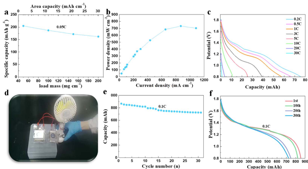
Fig. 4 (a) The discharge capacity of Fe-doped \alpha - \text{MnO}_2/\text{rGO} under high mass loadings ranging from 50 \text{ mg cm}^{-2} to 200 \text{ mg cm}^{-2} at 0.05C with the corresponding areal capacity. (b) The power density curve of Fe-doped \alpha - \text{MnO}_2/\text{rGO} under high mass loading. (c) The rate performance of the assembled pouch battery with a theoretical capacity of 100 mA h using Fe-doped \alpha - \text{MnO}_2/\text{rGO} as the cathode active material under a high mass loading of 180 \text{ mg cm}^{-2} . (d) The digital image of the commercial portable fans (4.5 W)-driven batteries by two connected assembled pouch batteries in series with 200 mA h. (e) The discharge curve of the assembled pouch battery with a theoretical capacity of 800 mA h at 0.1C and (f) the corresponding galvanostatic discharge profiles.
